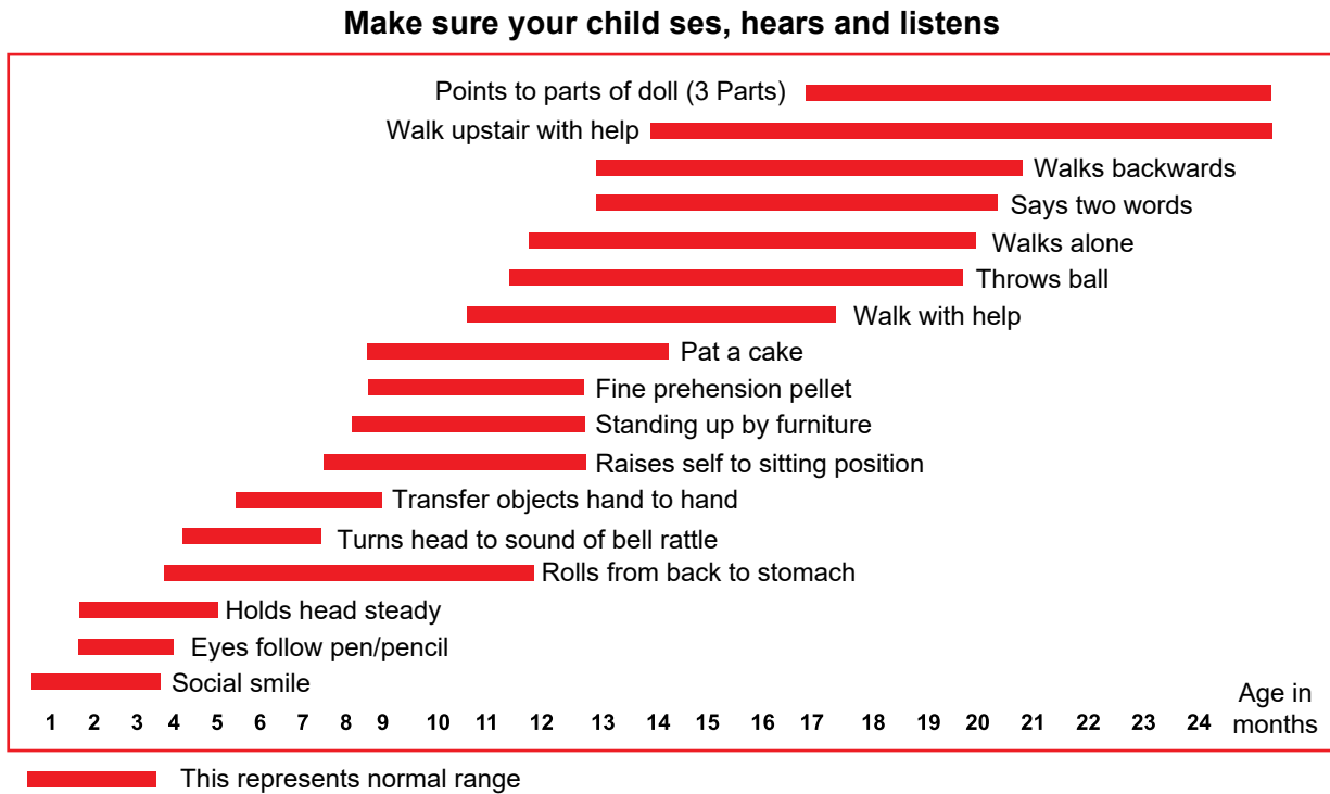
Figure 3.1.1: Development chart
