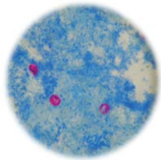
Figure 4.4.7: Cryptosporidium
