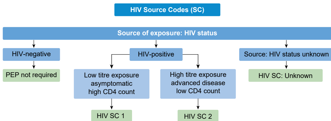
Figure 2.10.7: Source codes
